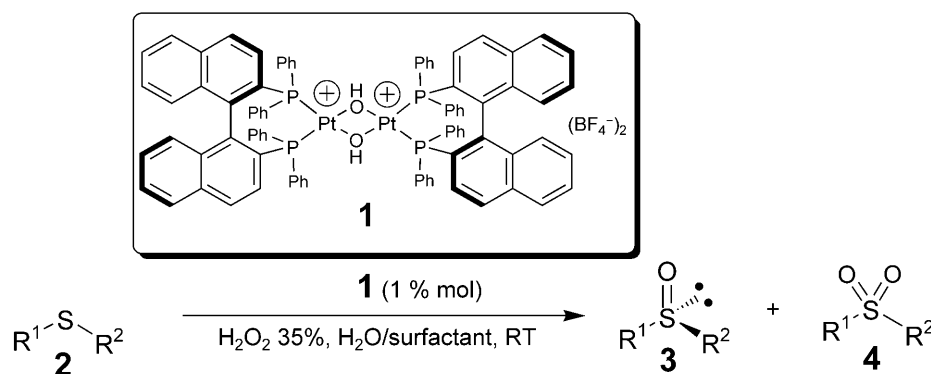
Scheme 1. \{[(R)\text{-BINAP}]\text{Pt}(\mu\text{-OH})_2(\text{BF}_4)_2 ( 1 )-catalyzed asymmetric sulfoxidation of prochiral aryl alkyl sulfides 2 with hydrogen peroxide in water with surfactants.
