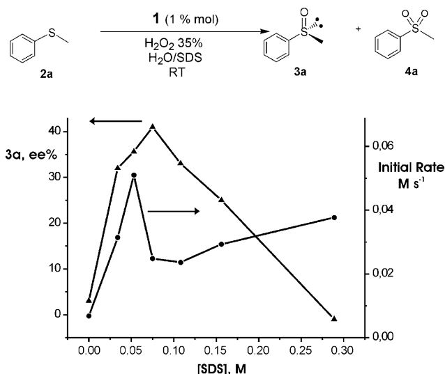
Figure 2. Effect of [SDS] on both enantiomeric excess (triangles) and initial rate (circles) for the asymmetric sulfoxidation of thioanisole ( 2a ) with hydrogen peroxide [substrate 2a : \text{H}_2\text{O}_2 : 1 = 100:100:1; [ 2a ] = 0.75 mmol, [ \text{H}_2\text{O}_2 ] = 0.75 mmol, [ 1 ] = 0.0075 mmol, solvent water 3 mL, sodium dodecyl sulfate SDS (75 mM, 1 mM in micelles), room temperature].
