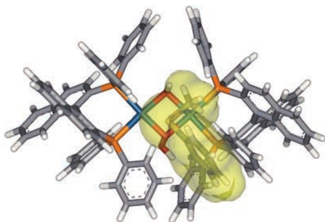
Figure 4. Postulated model for the approach of thioanisole ( 2a ) to the dimeric hydroperoxo active species. In particular, it is worth noting the proximity between the aromatic groups of the substrate and the complex and between the peroxidic oxygen and the sulfur atom of the thioether.
