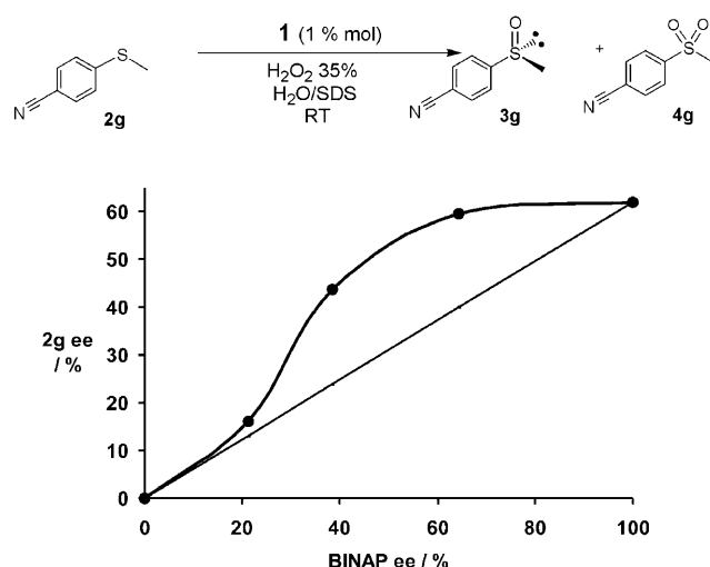
Figure 3. Positive non linear effect (+)-NLE for the oxidation of 2g with hydrogen peroxide catalyzed by 1 in diethyl ether/water-SDS biphasic system {substrate 2g :H 2 O 2 : 1 = 100:100:1; [ 2g ] = 0.75 mmol, [H 2 O 2 ] = 0.75 mmol, [ 1 ] = 0.0075 mmol, solvent water 3 mL, sodium dodecyl sulfate SDS (75 mM, 1 mM in micelles), room temperature}.
