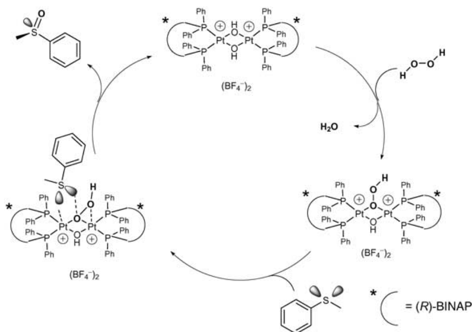
Scheme 2. Possible catalytic mechanistic cycle for the oxidation of aryl alkyl sulfides with hydrogen peroxide mediated by 1 in water-SDS.
