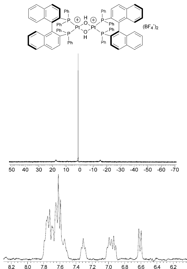
Figure 1. NMR spectra: ^{31}\text{P}\{^1\text{H}\} (top) and ^1\text{H} NMR spectra (bottom) of [(R)\text{-BINAP}]\text{Pt}(\mu\text{-OH})_2(\text{BF}_4)_2 ( 1 ). [ 1 ] = 2.5 mM, [SDS] = 75 mM in \text{H}_2\text{O}/\text{D}_2\text{O} (75/25).
