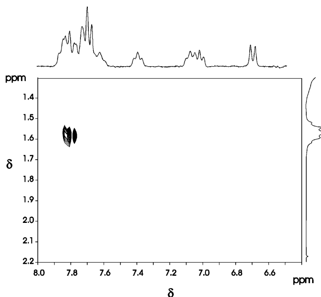
Figure 5. Portion of the 2D NOESY spectrum of \{[(R)\text{-BINAP}]\text{Pt}(\mu\text{-OH})_2(\text{BF}_4)_2\} ( 1 ), [ 1 ] = 2.5 mM, [SDS] = 75 mM in H 2 O/D 2 O (75/25), showing the cross-peak between the catalyst and the second methylene of SDS.
